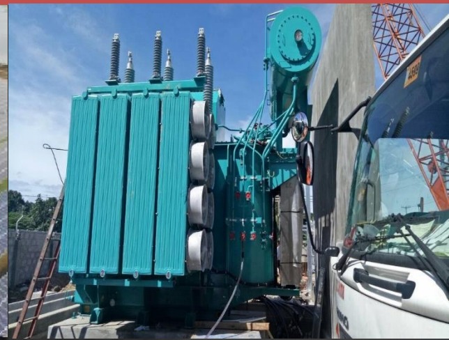
SUPPLY AND DELIVERY OF 30/40/50MVA 69/13.8kv POWER TRANSFORMER & SPARE PARTS (PTCG BRAND) CLIENT: CLARK ELECTRIC DISTRIBUTION CORPORATION (CEDC) LOCATION: ANGELES, PAMPANGA SCOPE OF WORKS: ELECTRICAL WORKS
