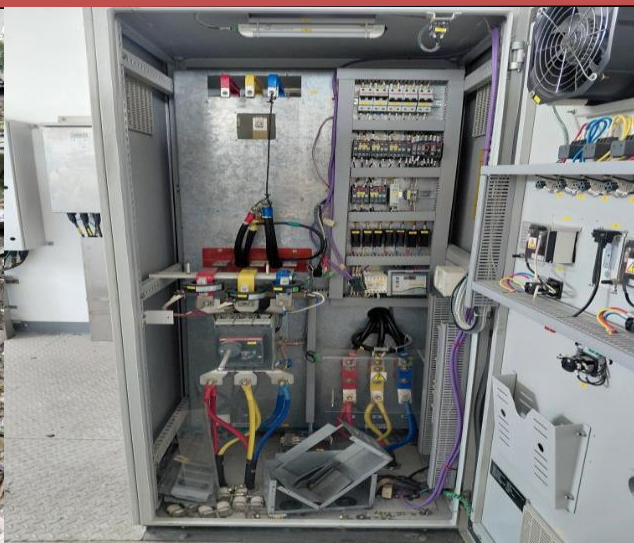
SUPPLY AND INSTALL OF SOFT STARTER @ ILLUGIN STP
