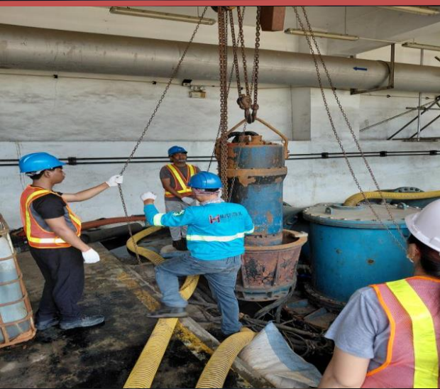
REWINDING AND REFURBISHMENT OF 132 KW SUBMERSIBLE PUMP 1 @ LKK STP
